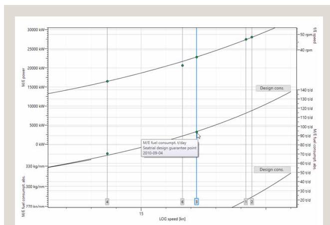
Verification of consumption during sea-trial against design.
